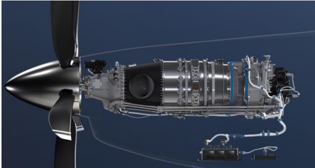
Full Digital Control of the Engine & the Propeller
